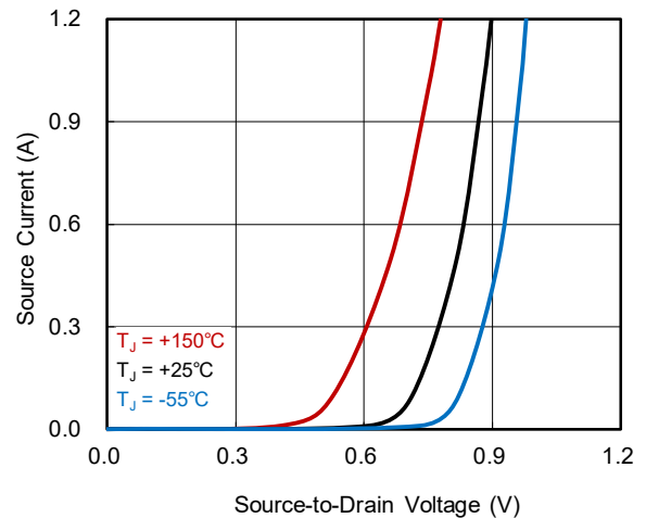
Diode Forward
