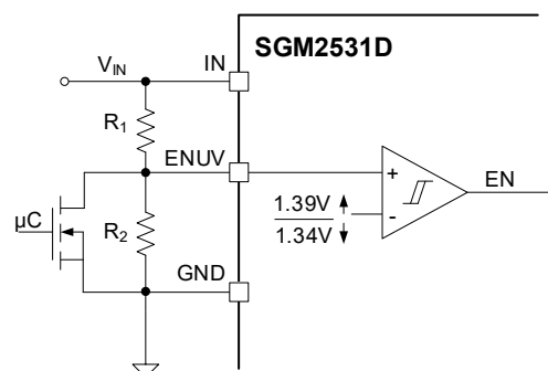
Figure 8. Shutdown Control
