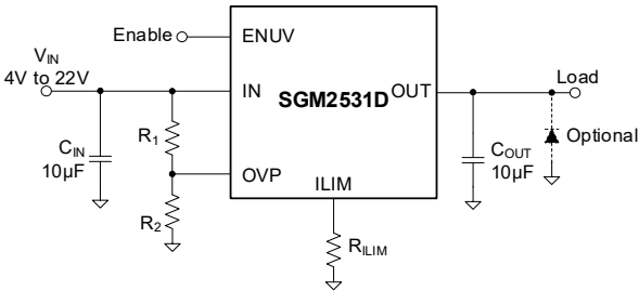
Figure 9. Smart Load Switch Implementation
