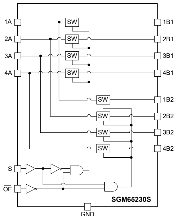
Figure 1. Block Diagram
