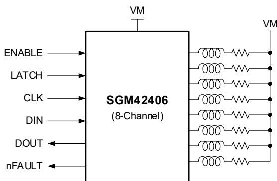
Figure 1. Simplified Schematic
