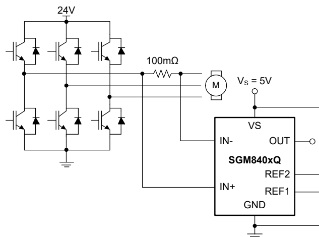
Figure 12. In-Line Motor Current Measurement
