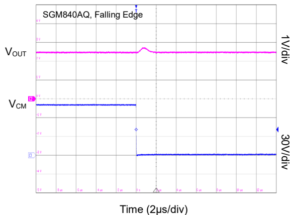
Common-Mode Voltage Transient Response
