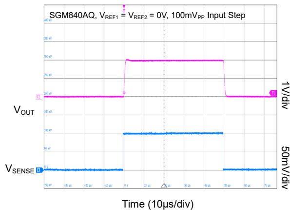
Step Response
