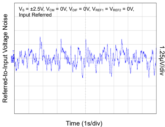
0.1Hz to 10Hz Voltage Noise
