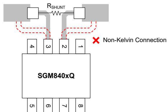
Figure 16. Shunt Connections to the SGM840xQ
