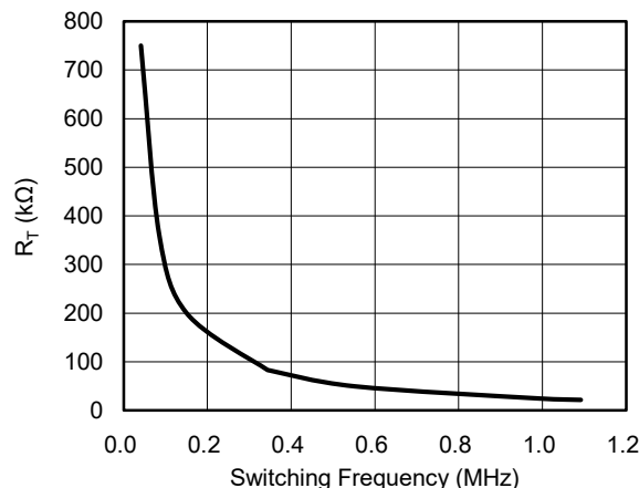
Figure 3. R_T and Switching Frequency Relationship
