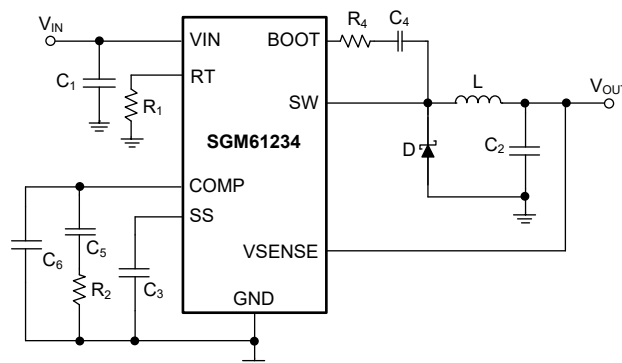
Figure 4. SGM61234 Typical Application Circuit
