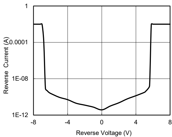
IV Curve
