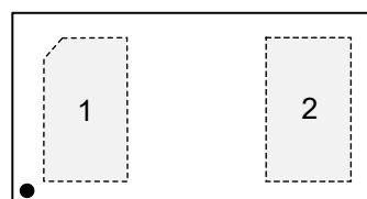
UTDFN-1×0.6-2AL
