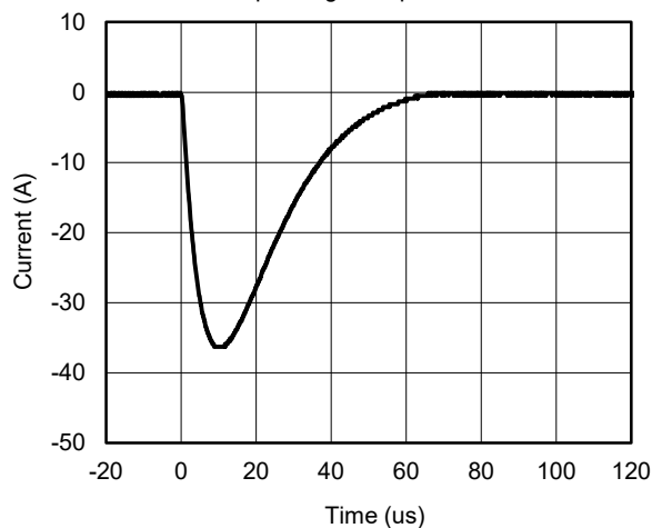
8/20 \mu s Surge Response at -36A
