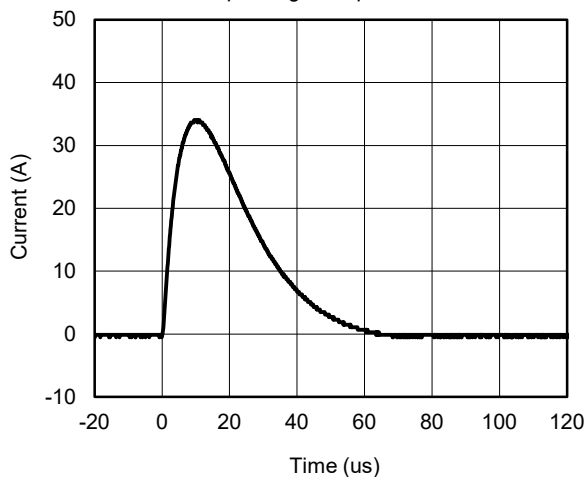
8/20 \mu s Surge Response at 34A
