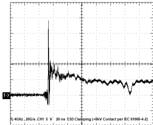
IEC61000-4-2 Contact +8kV
