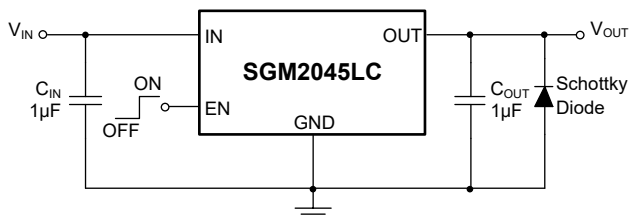
Figure 4. Negatively Biased Output Application
