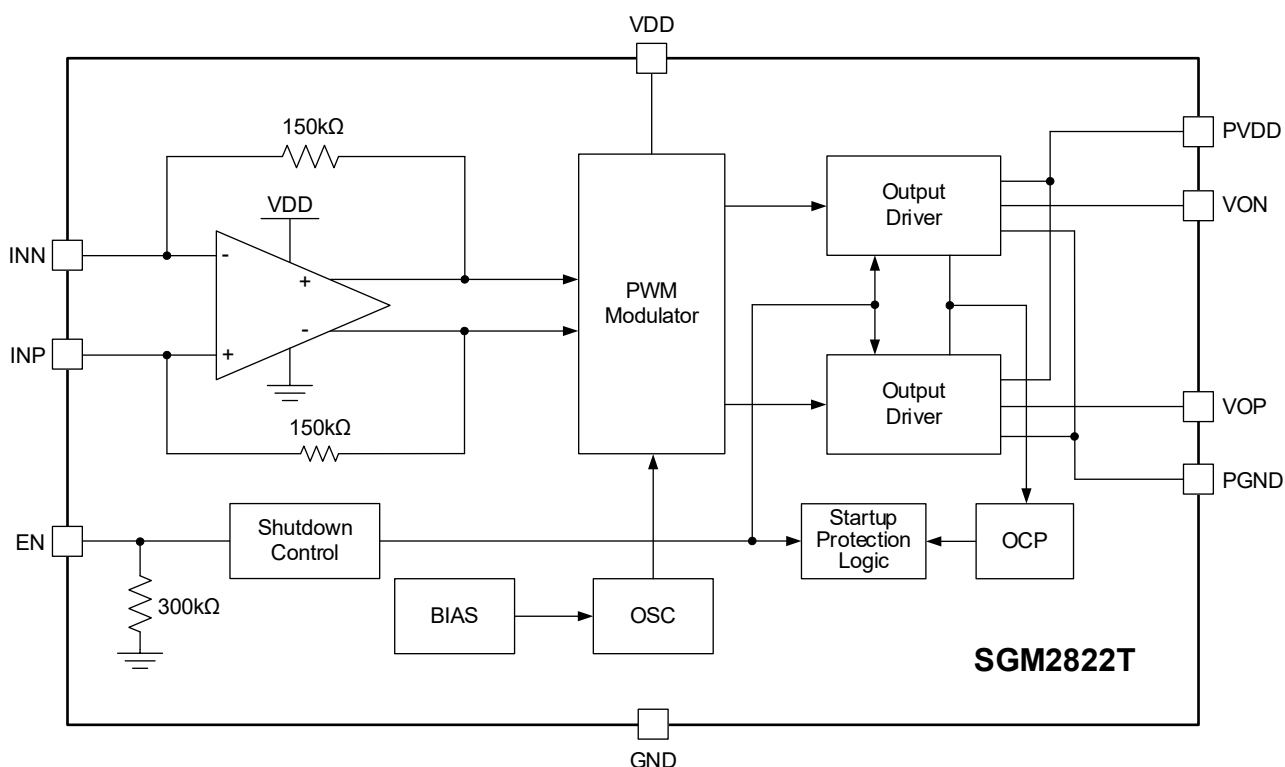
Figure 3. Simplified Function Block Diagram of SGM2822T
