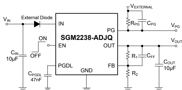
Figure 7. Reverse Protection Reference Design
