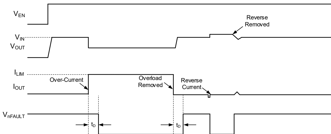
Figure 4. Fault Timing: Output Reset by Toggling EN
