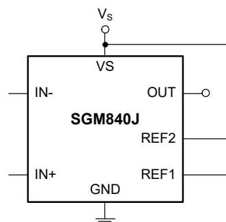
Figure 6. VS Referenced Output
