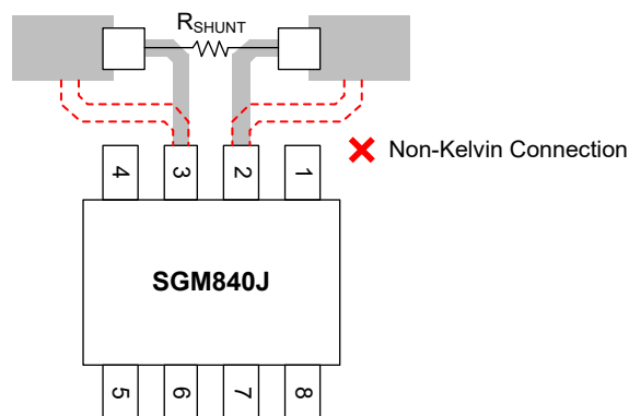
Figure 12. Shunt Connections to the SGM840J
