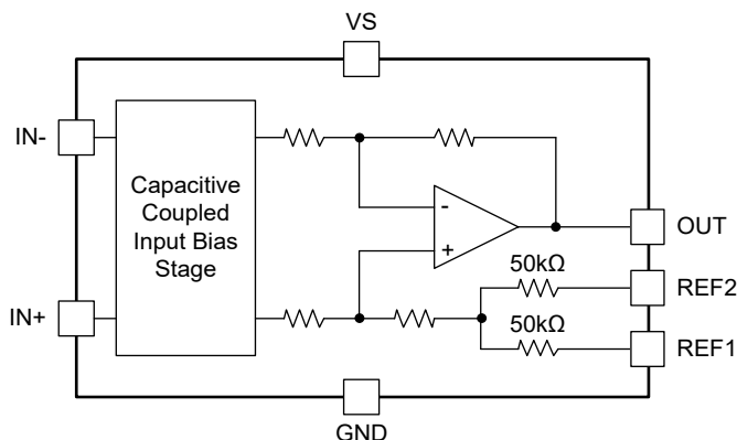
Figure 2. Block Diagram
