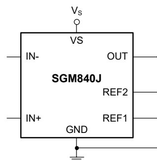
Figure 5. GND Referenced Output
