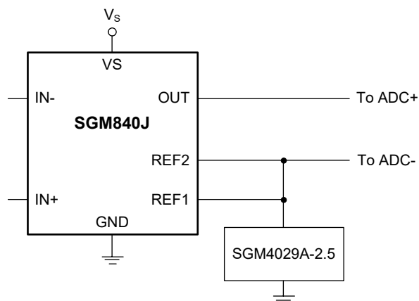
Figure 10. Reference Different Output
