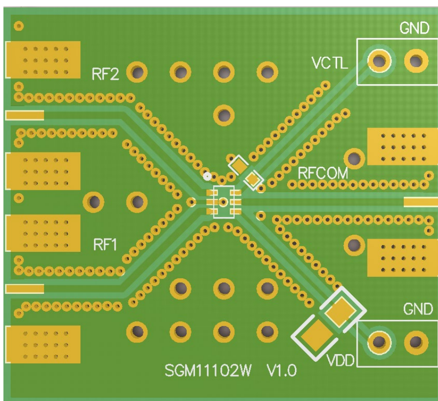
Figure 3. SGM11102W Evaluation Board Layout
