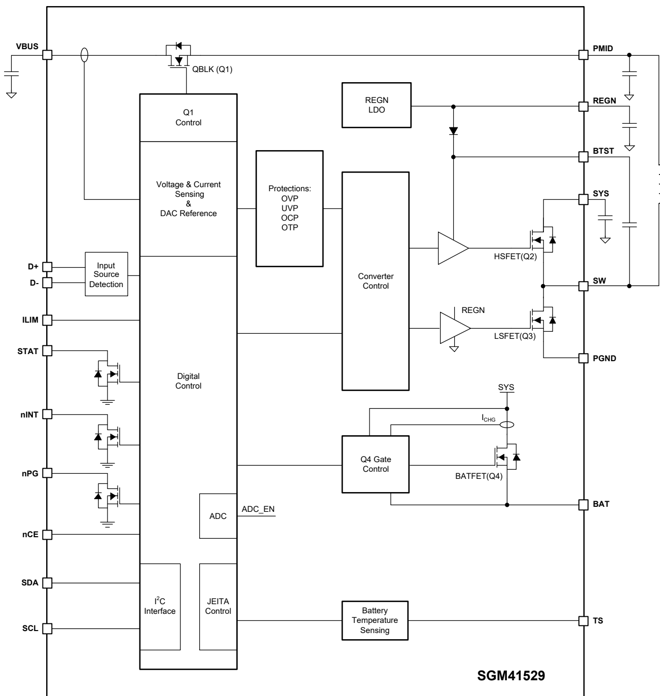
Figure 2. Block Diagram
