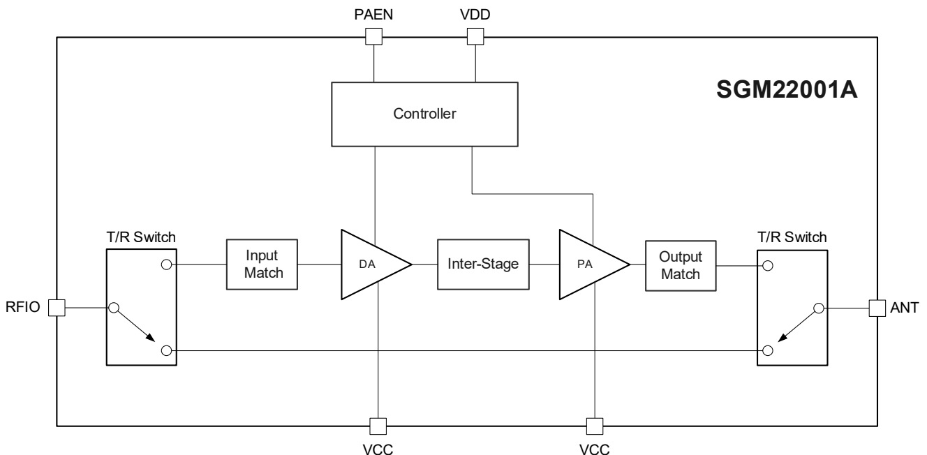
Figure 1. SGM22001A Block Diagram
