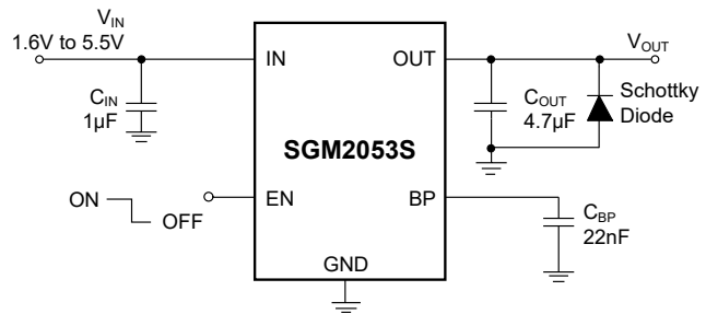
Figure 9. Negatively Biased Output Application
