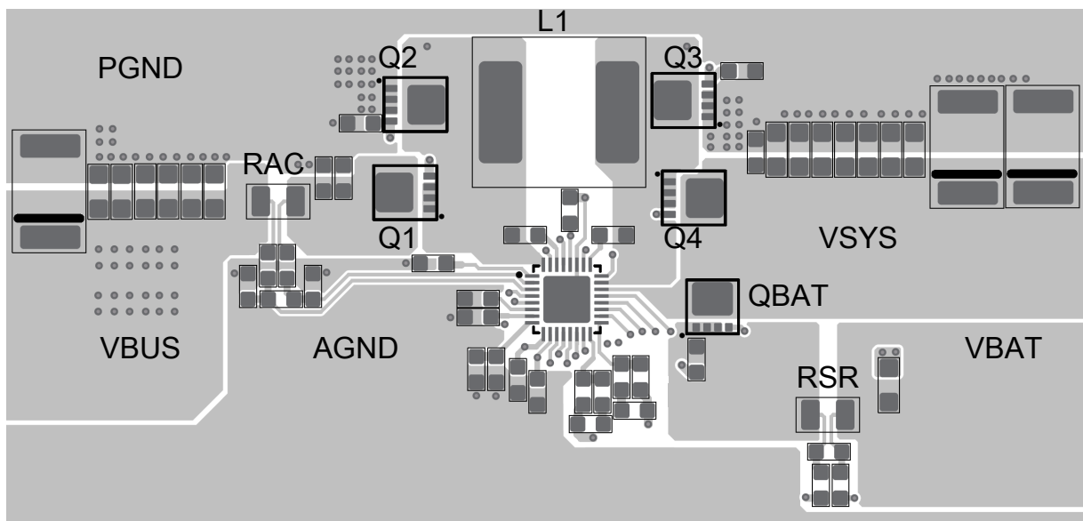
Figure 9. PCB Layout Example
