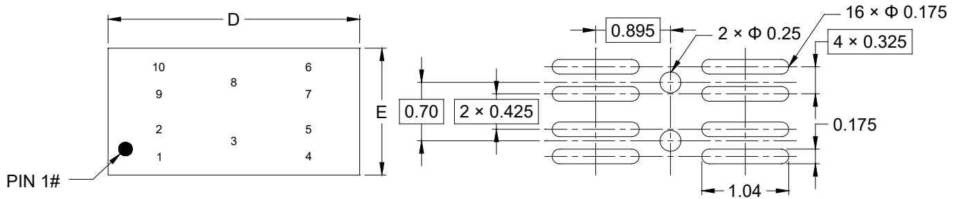
RECOMMENDED LAND PATTERN (Unit: mm)
