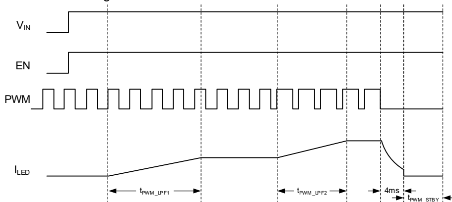
Figure 4. Enabling the SGM37360A via PWM
