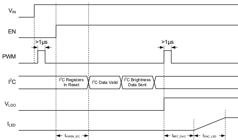
Figure 5. Enabling the SGM37360A via I 2 C
