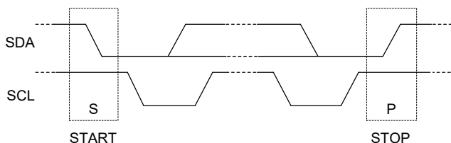
Figure 15. I 2 C Start and Stop Conditions
