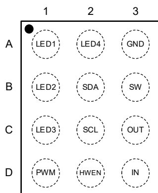
SGM37604S (TOP VIEW)
