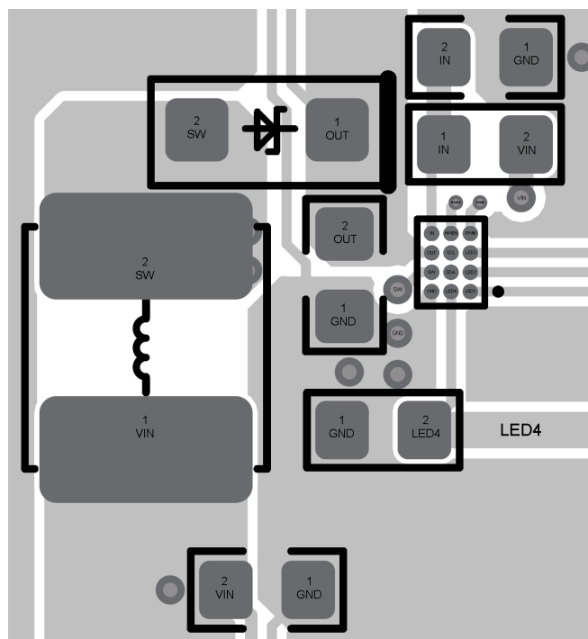
Figure 17. Layout Example
