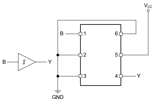
Figure 7. Buffer
