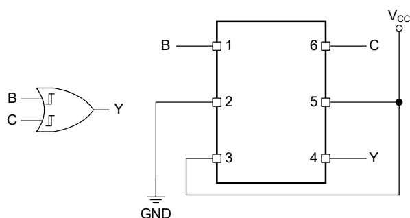
Figure 5. 2-Input OR Gate
