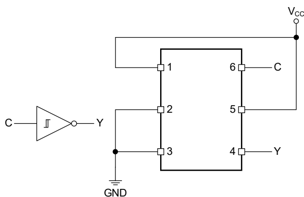
Figure 6. Inverter
