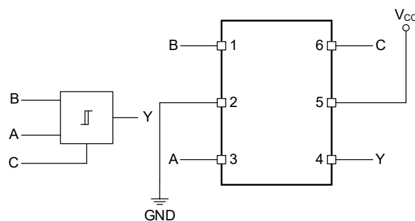
Figure 1. 2-Input MUX
