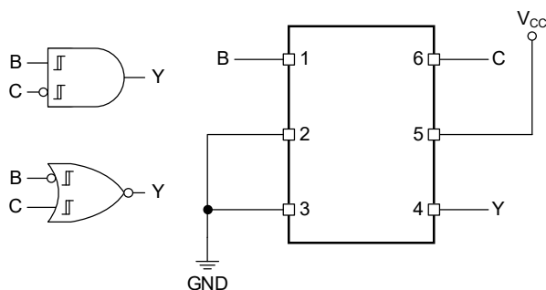
Figure 4. 2-Input AND Gate with Inverted Input C or 2-Input NOR Gate with Inverted Input B
