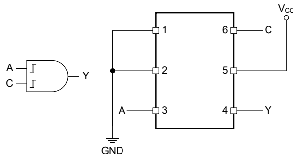
Figure 2. 2-Input AND Gate
