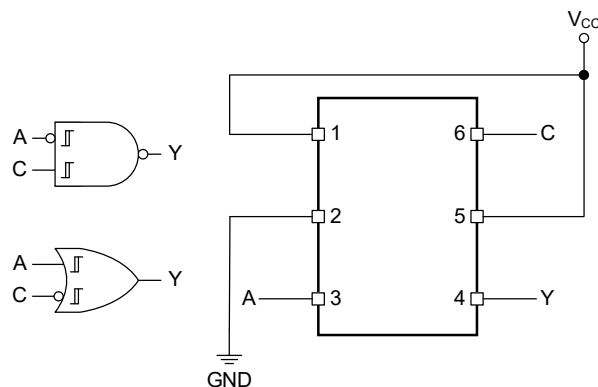
Figure 3. 2-Input NAND Gate with Inverted Input A or 2-Input OR Gate with Inverted Input C
