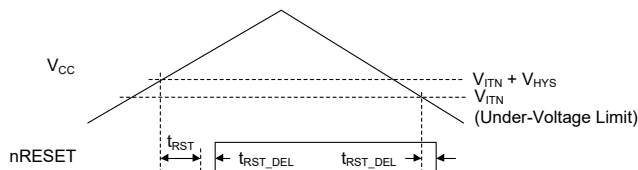
Figure 5. Under-Voltage Detection
