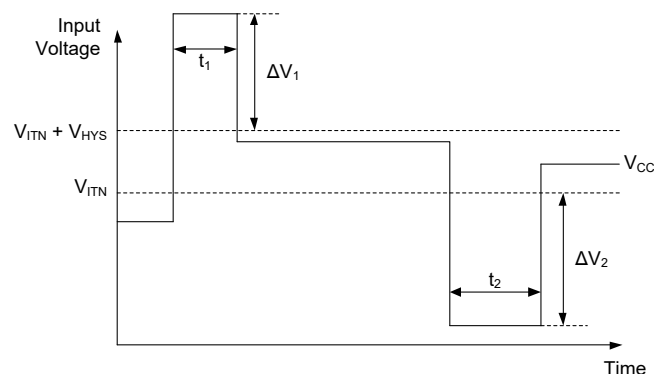
Figure 9. Overdrive Voltage
