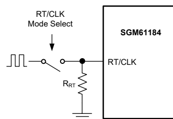
Figure 5. Using RT and CLK Modes Together
