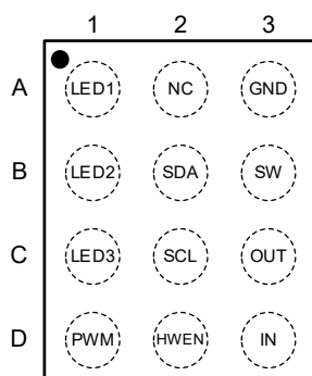
SGM37603S (TOP VIEW)
