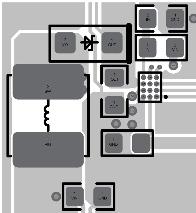
Figure 17. Layout Example
