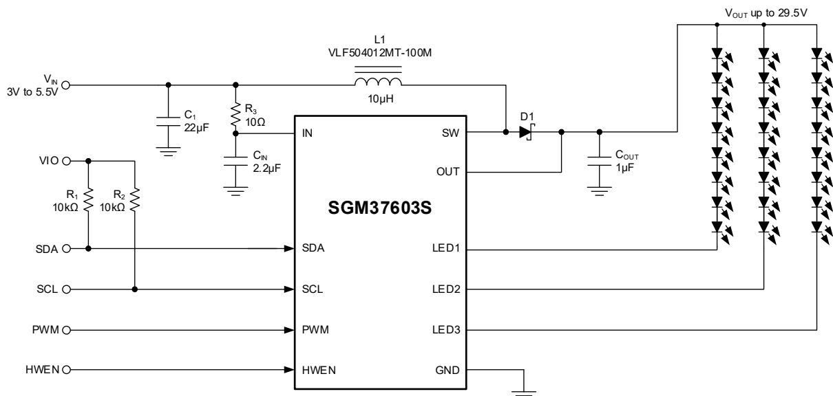
Figure 1. Typical Application
