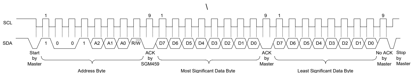
(a) 2-Byte Read from Preset Pointer Location Such as Temperature, T_{OS} and T_{HYST}
