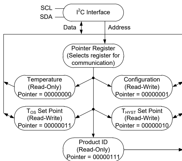
Figure 8. Register Structure
