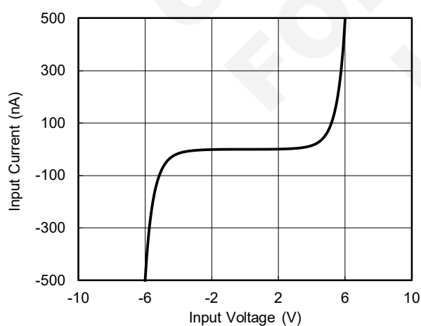
IV Curve
