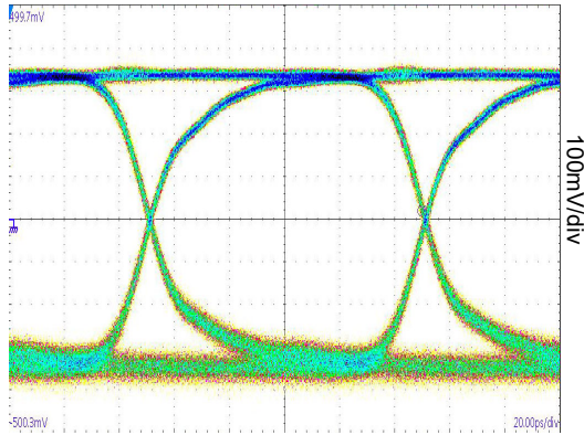
USB3.x Eye Diagram without SGM05FB8D2 10Gbps, 800mVpp, Test Board Only
