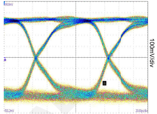
USB3.x Eye Diagram with SGM05FB8D2 10Gbps, 800mVpp, Test Board + SGM05FB8D2
