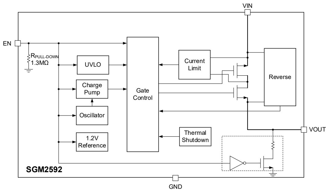
Figure 2. Block Diagram
