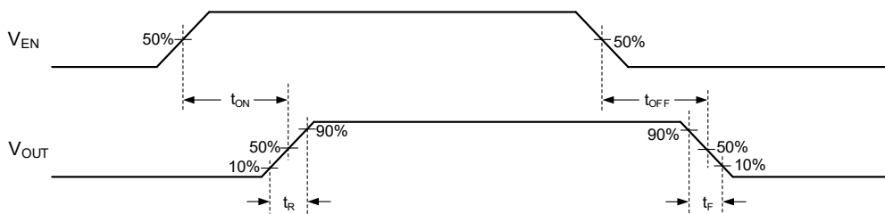
Figure 3. Switch Turn-On and Turn-Off Delay Times
