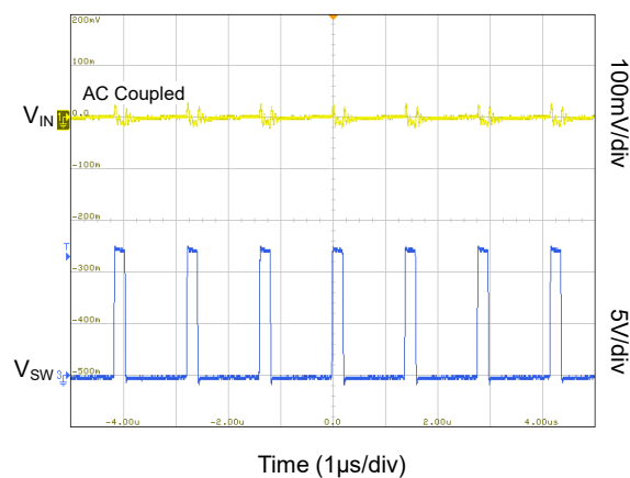
V_{IN} Ripple No Load (SGM611A14B)
