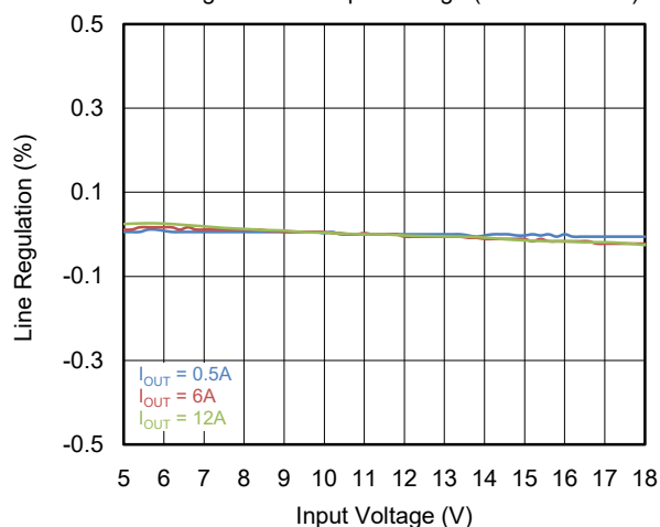
Line Regulation vs. Input Voltage (SGM611A14B)
