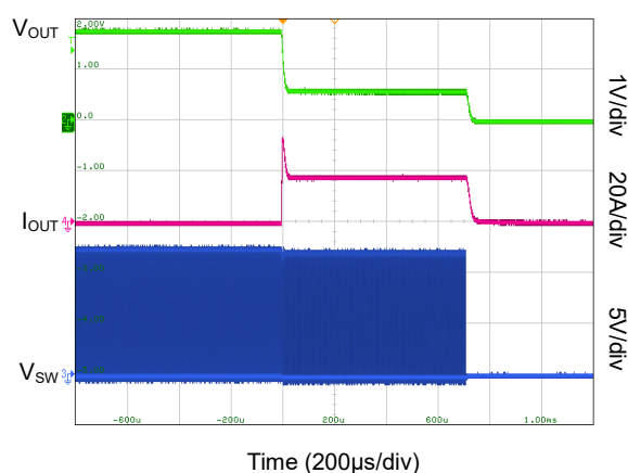
Short-Circuit (SGM611A14B)
