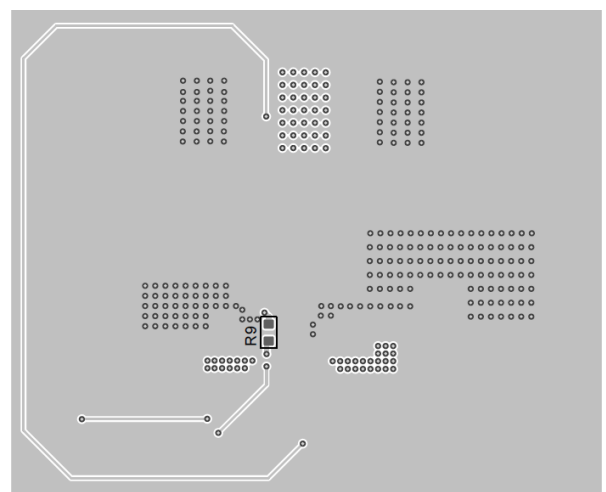
Figure 15. Bottom Layer
