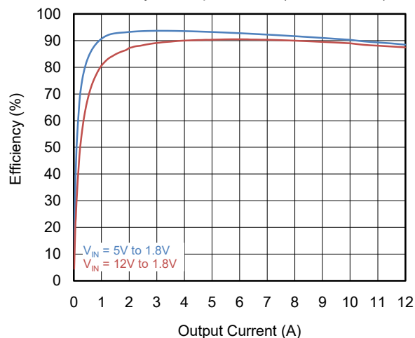
Efficiency vs. Output Current (SGM611A14B)
