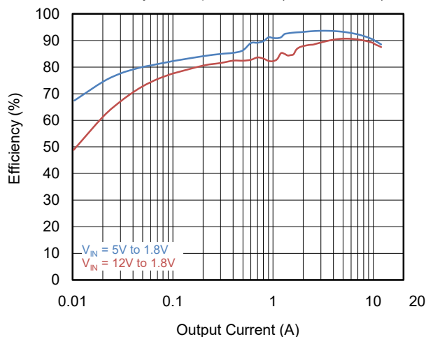
Efficiency vs. Output Current (SGM611A14A)
