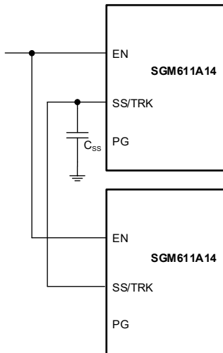
Figure 9. Ratiometric Sequencing of Two Devices
