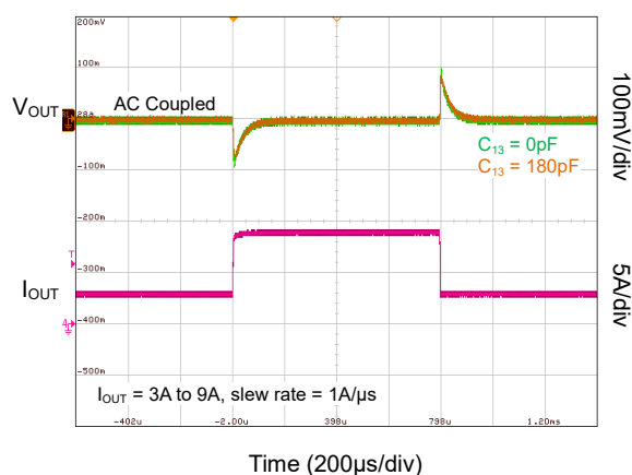
Load Transient Response (SGM611A14B)
