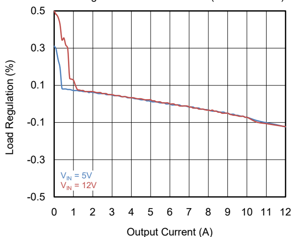
Load Regulation vs. Load Current (SGM611A14A)
