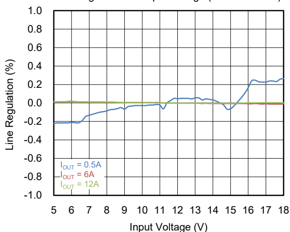
Line Regulation vs. Input Voltage (SGM611A14A)
