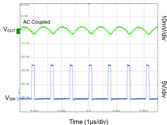
V_{OUT} Ripple 0A (SGM611A14B)
