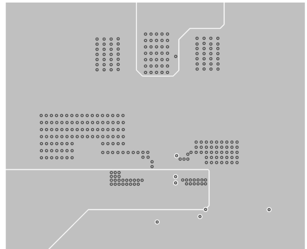
Figure 14. Mid Layer 2
