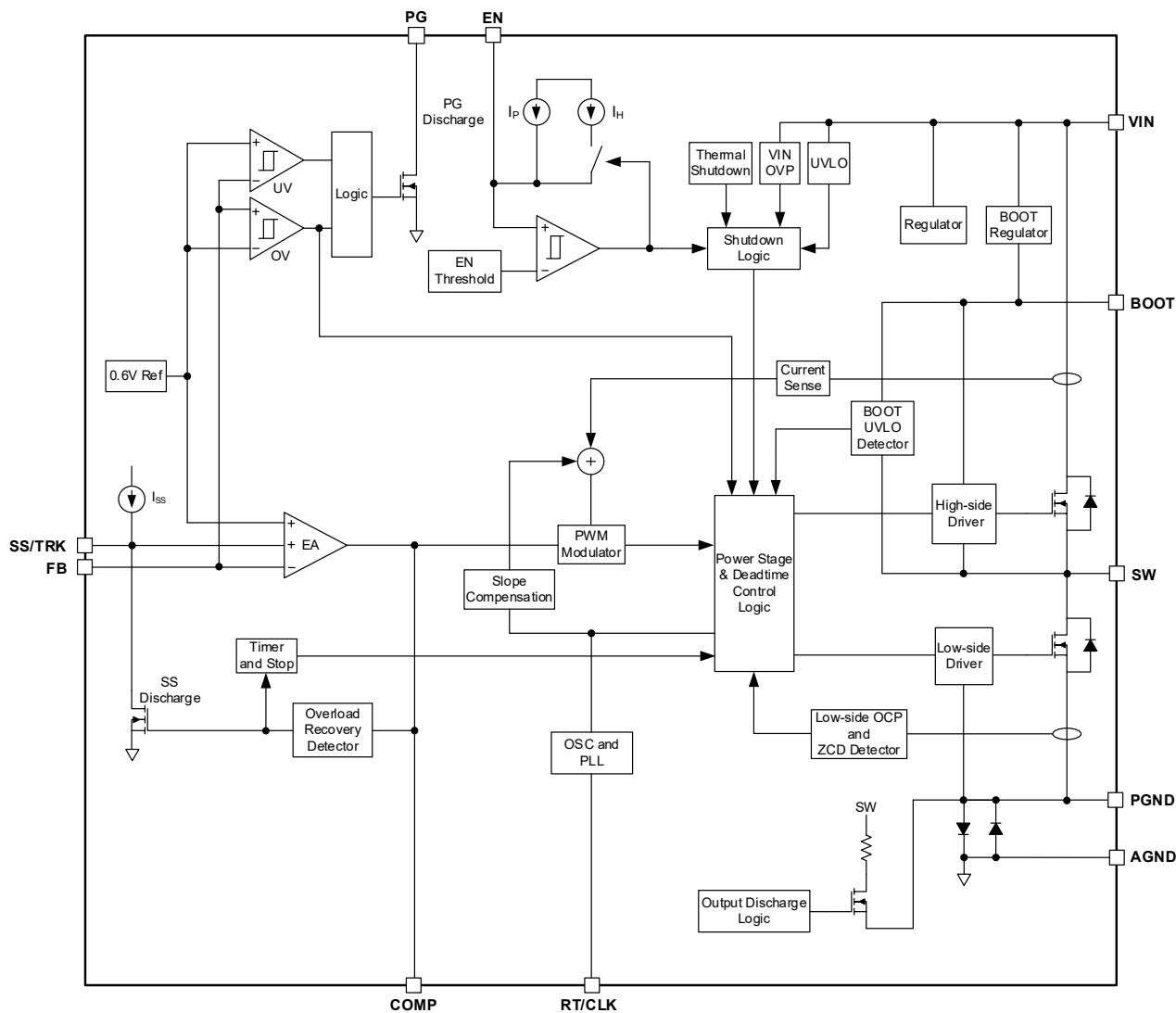
Figure 2. Block Diagram
