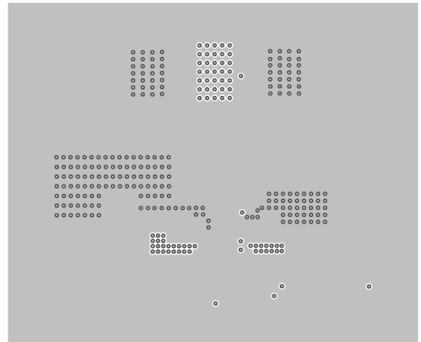
Figure 13. Mid Layer 1
