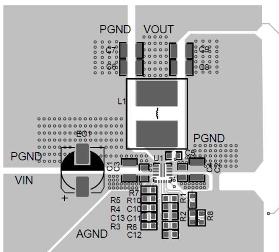
Figure 12. Top Layer
