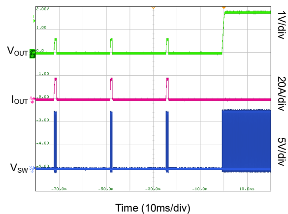
Hiccup Recovery (SGM611A14B)
