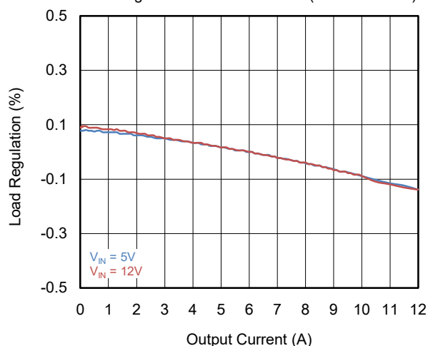
Load Regulation vs. Load Current (SGM611A14B)
