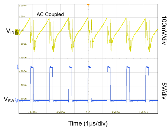
V_{IN} Ripple Full Load (SGM611A14A/B)
