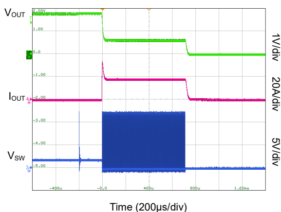
Short-Circuit (SGM611A14A)
