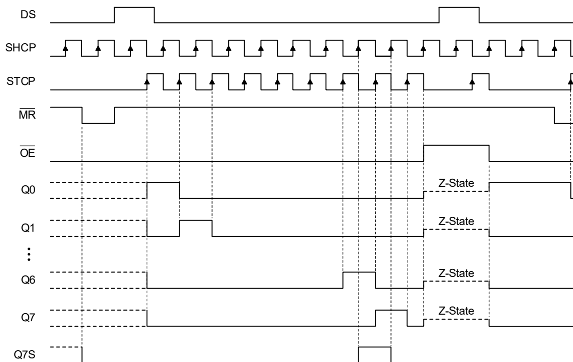
Figure 1. Timing Diagram
