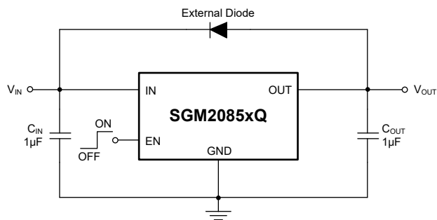
Figure 6. Reverse Protection Reference Design
