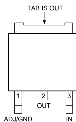
TO-252-2A
