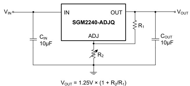
Adjustable Voltage Typical Application Circuit
