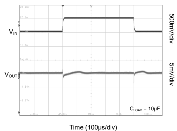
Line Transient
