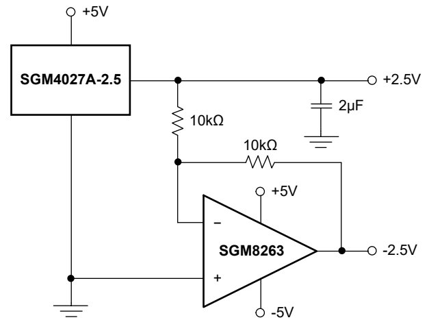
Figure 4. Positive and Negative Voltage Reference
