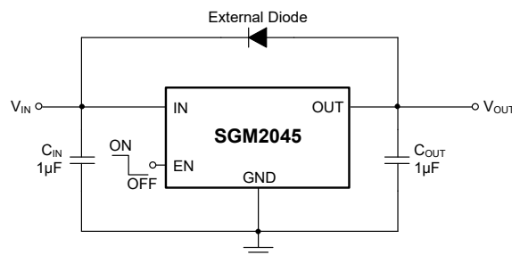
Figure 3. Reverse Protection Reference Design
