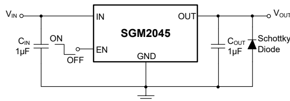
Figure 4. Negatively Biased Output Application
