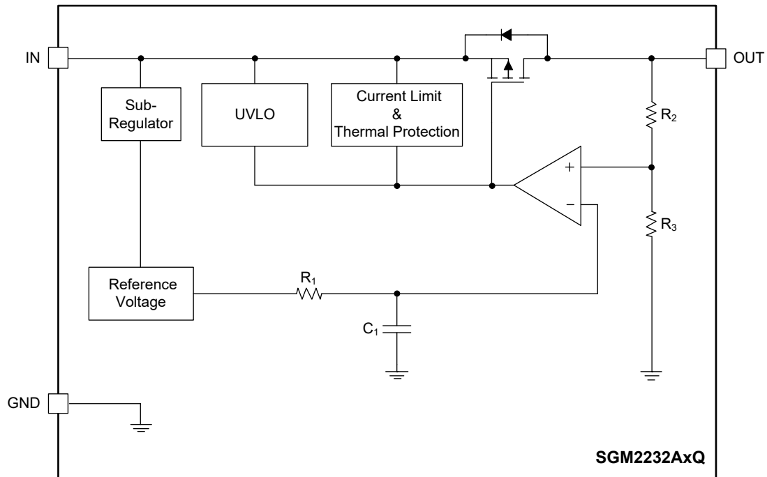
Figure 2. Block Diagram
