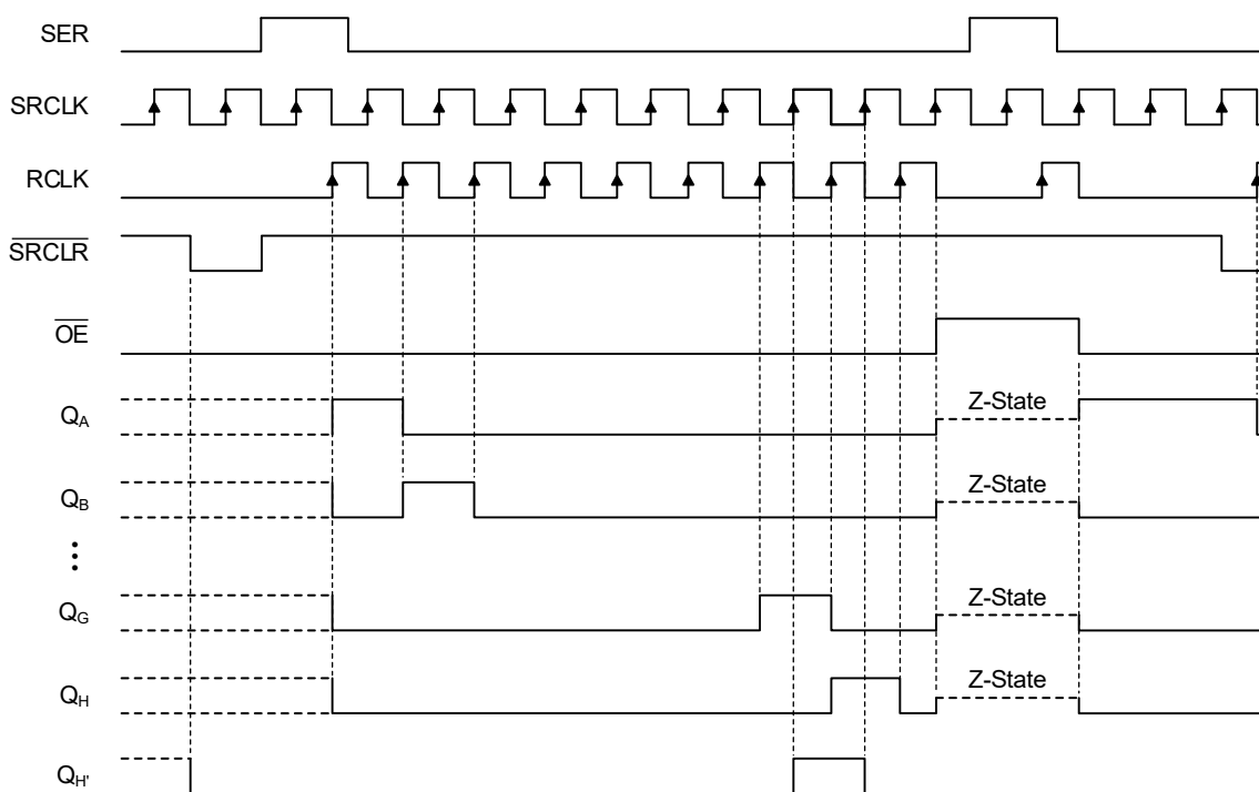
Figure 1. Timing Diagram
