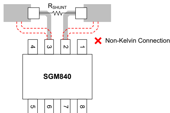
Figure 16. Shunt Connections to the SGM840
