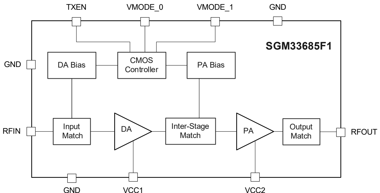
Figure 1. SGM33685F1 Block Diagram
