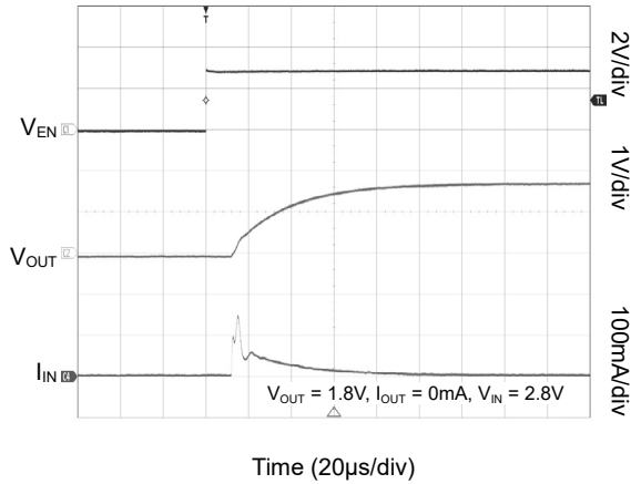
Turn On Speed with EN Pin
